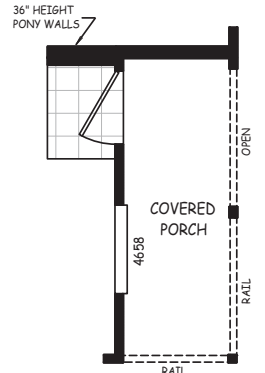
ALT FRONT DOOR LOCATION
