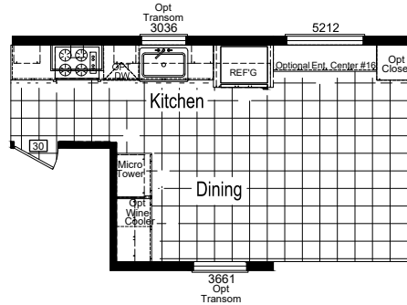
OPTIONAL ULTIMATE KITCHEN 2 AVAILABLE 9FT FLAT ONLY
